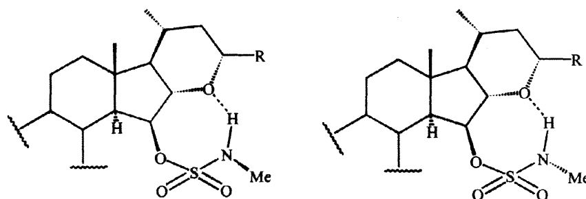
Figure 2. The two isomers present as a result of the sulfamate functionality
